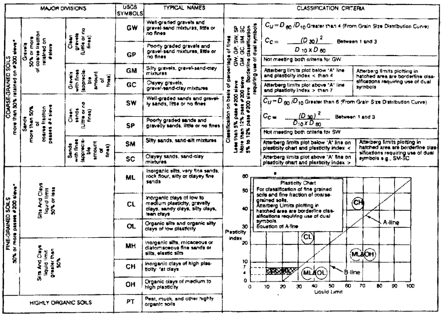
Figure 1-1. Unified soil classification system criteria
